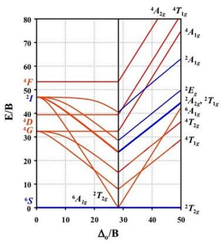
d^5 Tanabe-Sugano Diagram
