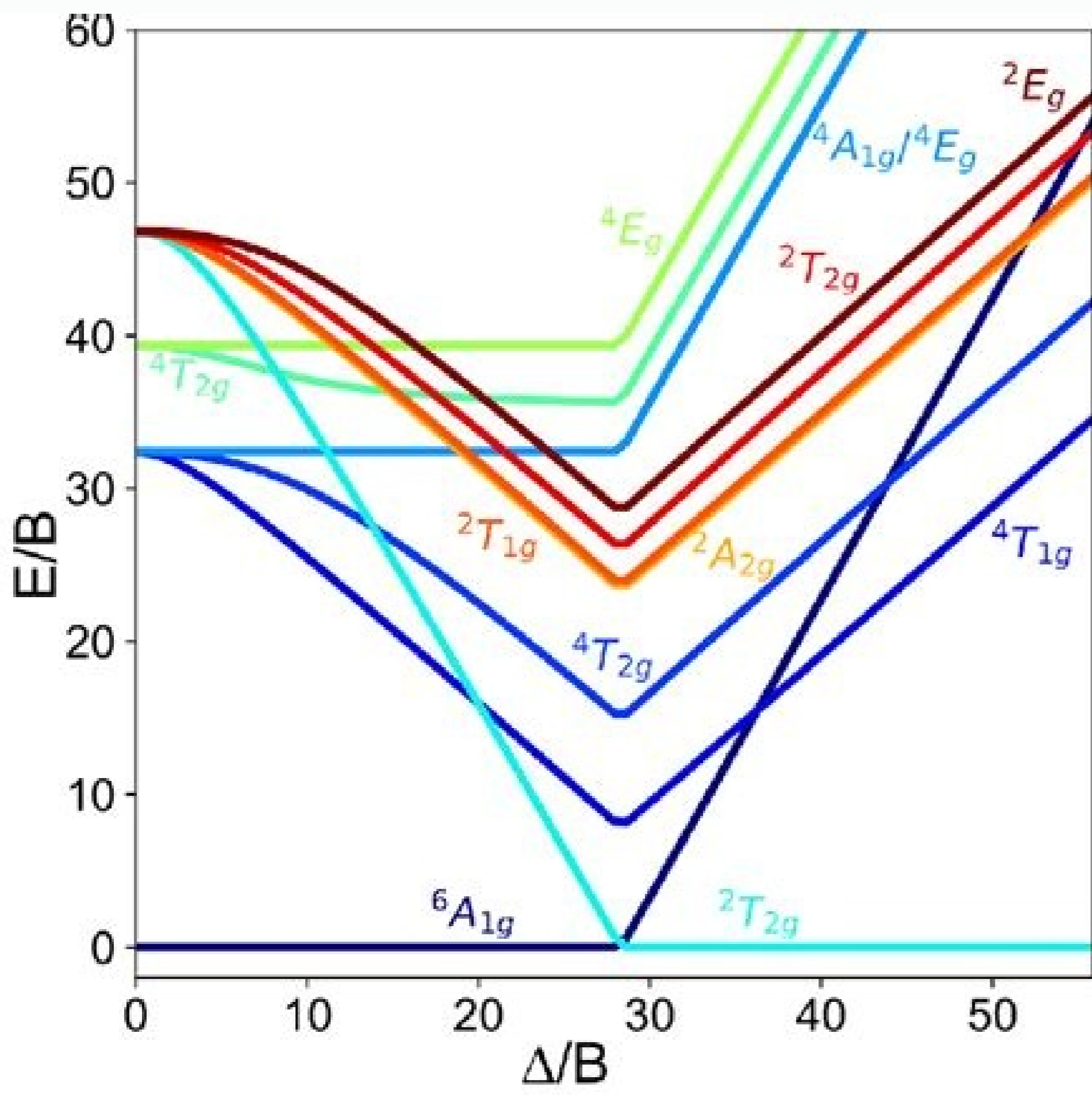
d^5 Tanabe-Sugano Diagram
